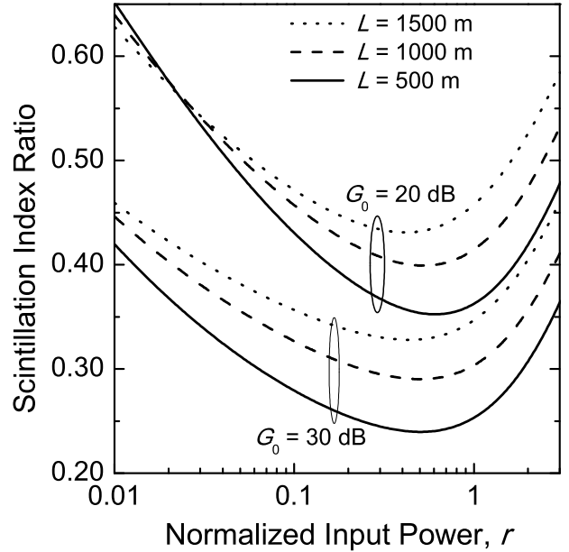
Fig. 4. Scintillation index ratio \frac{\sigma_u}{\sigma_\gamma - \gamma} versus the normalized input power r .
