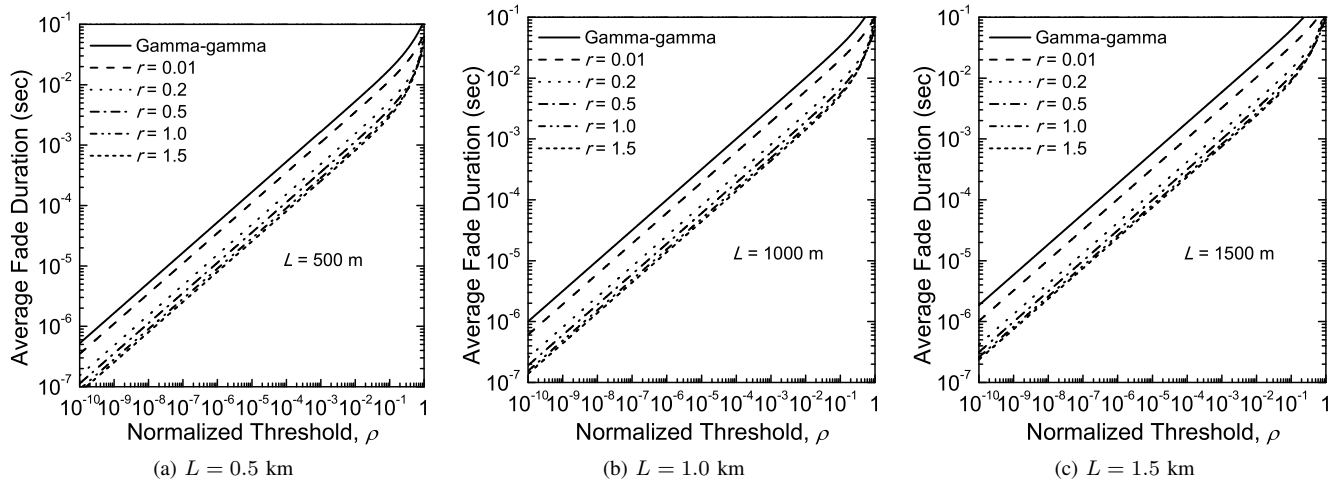
Fig. 5. Average fade duration at the output of the SOA versus the normalized threshold \rho for G_0 = 20 dB and L = 0.5, 1.0 and 1.5 km.
