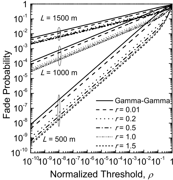
Fig. 3. Fade probability at the output of the SOA versus the normalized threshold \rho for SOA small signal gain G_0 = 20 dB.
