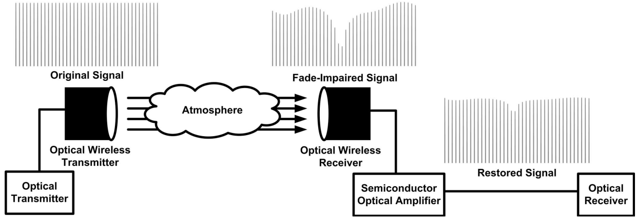
Fig. 1. Principle of operation of the proposed technique.
