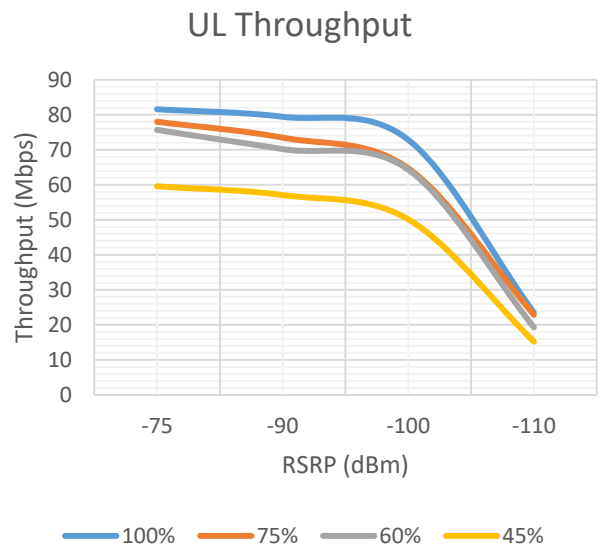
Fig. 8 Throughput of the uplink channel
