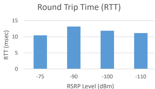
Fig. 5 Round trip time of reference system
