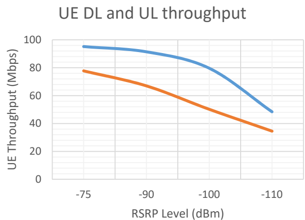
Fig. 4 UE throughput for downlink and uplink channel
